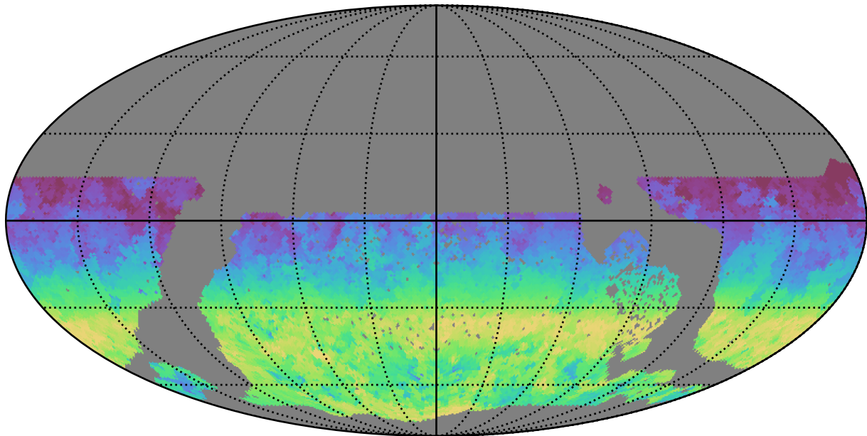
too_5_1v3.4_10yrs WFD z band: AngleRange rotSkyPos
