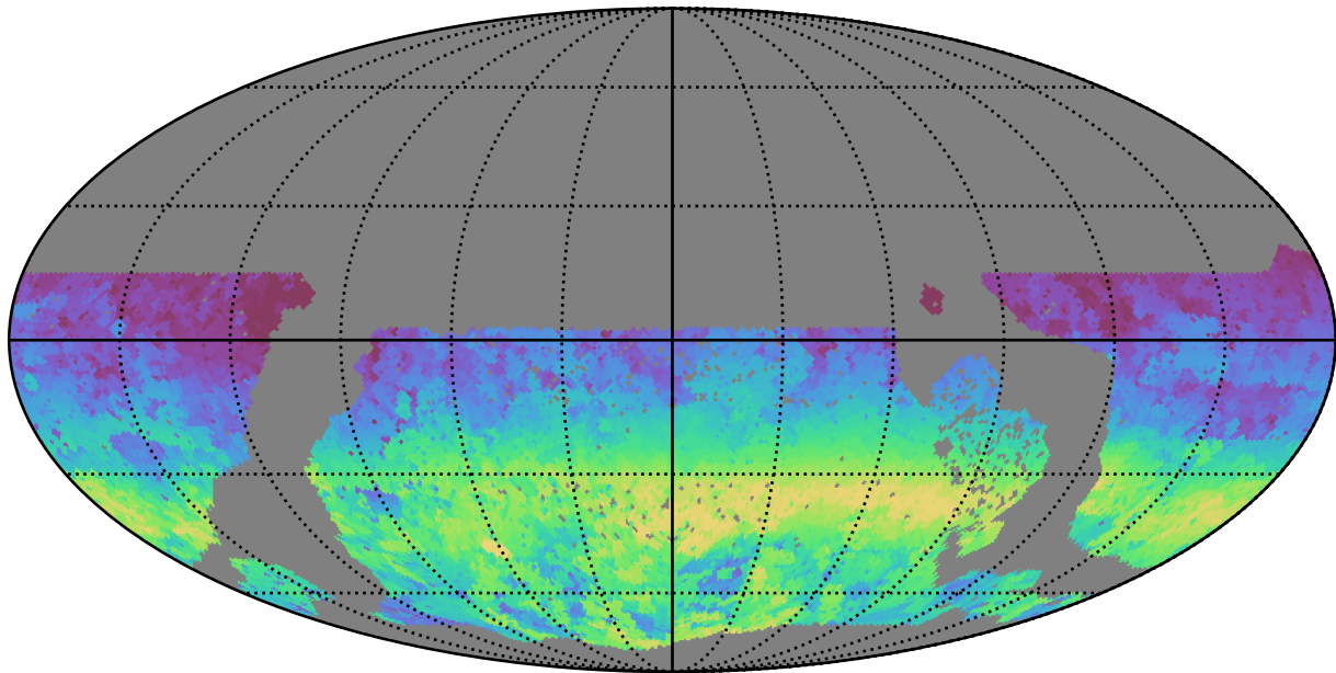
too_5_1v3.4_10yrs WFD y band: AngleRange rotSkyPos
