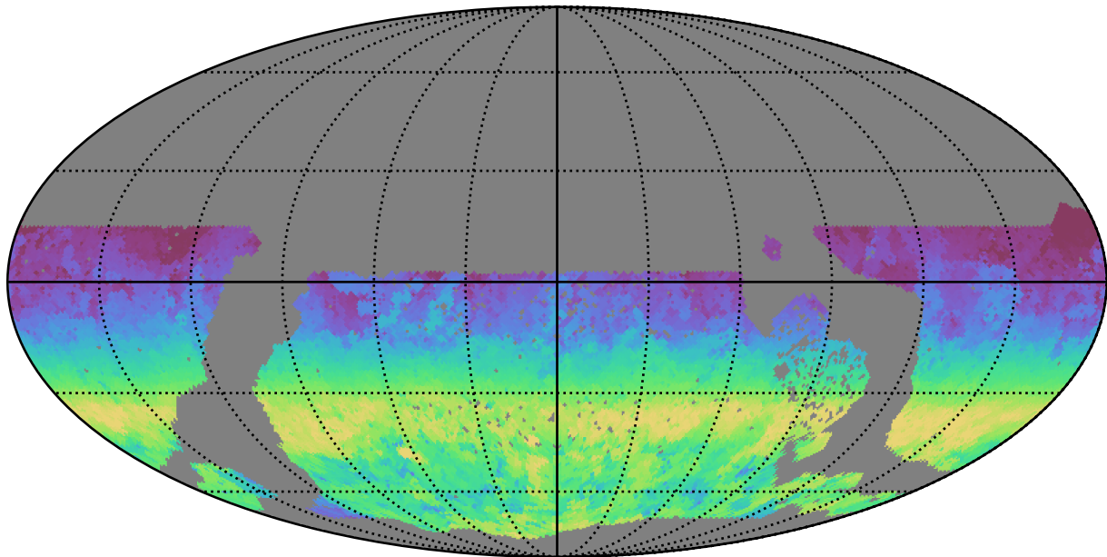
too_5_1v3.4_10yrs WFD r band: AngleRange rotSkyPos
