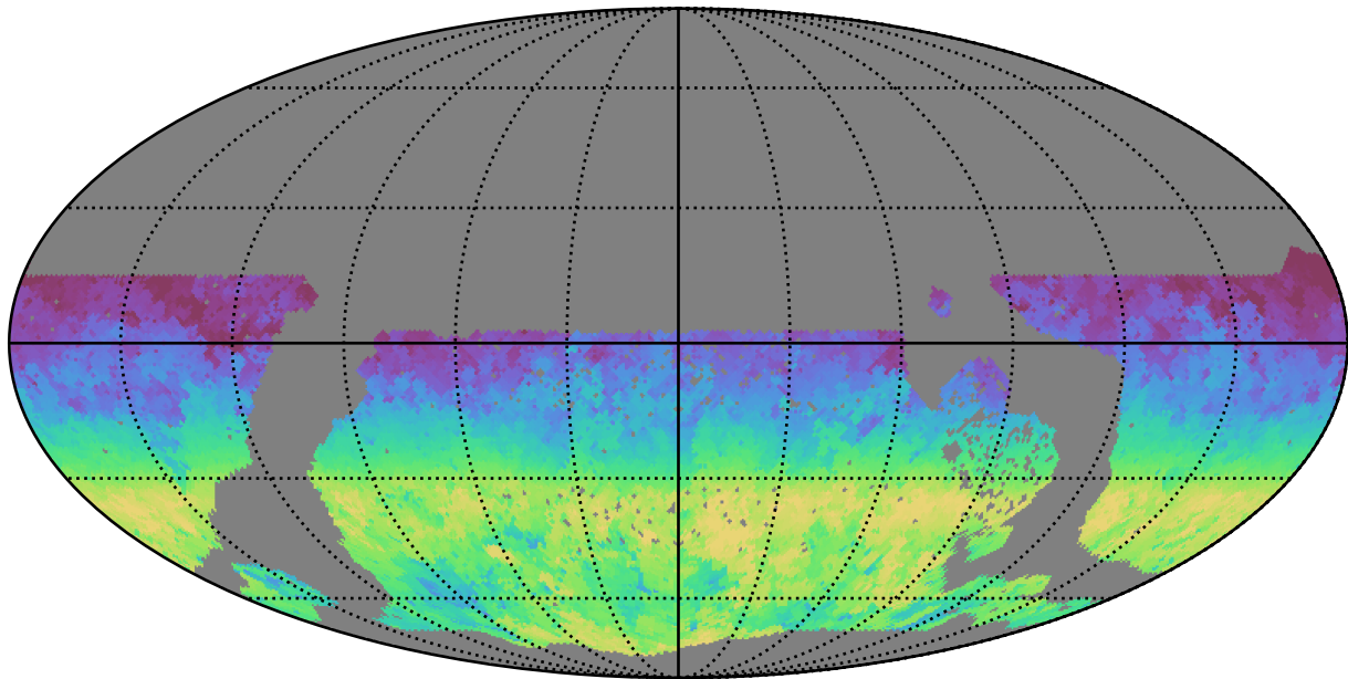
too_5_1v3.4_10yrs WFD i band: AngleRange rotSkyPos
