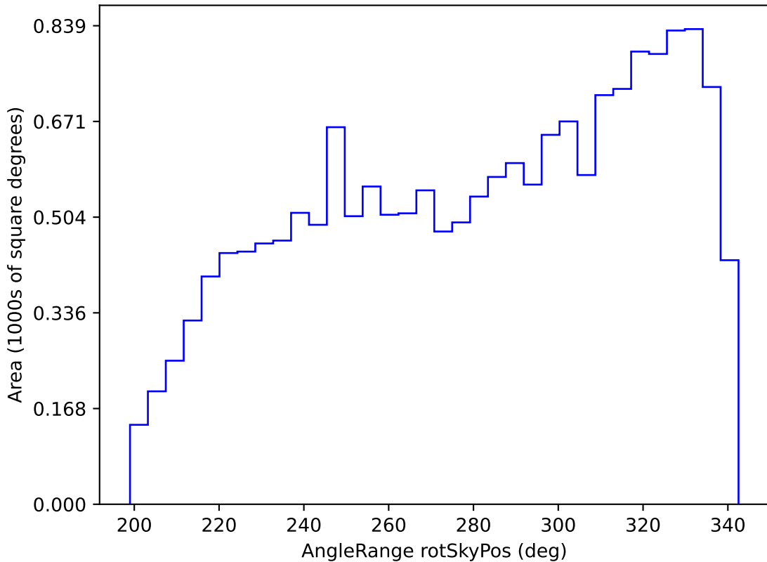
too_5_1v3.4_10yrs WFD i band: AngleRange rotSkyPos
