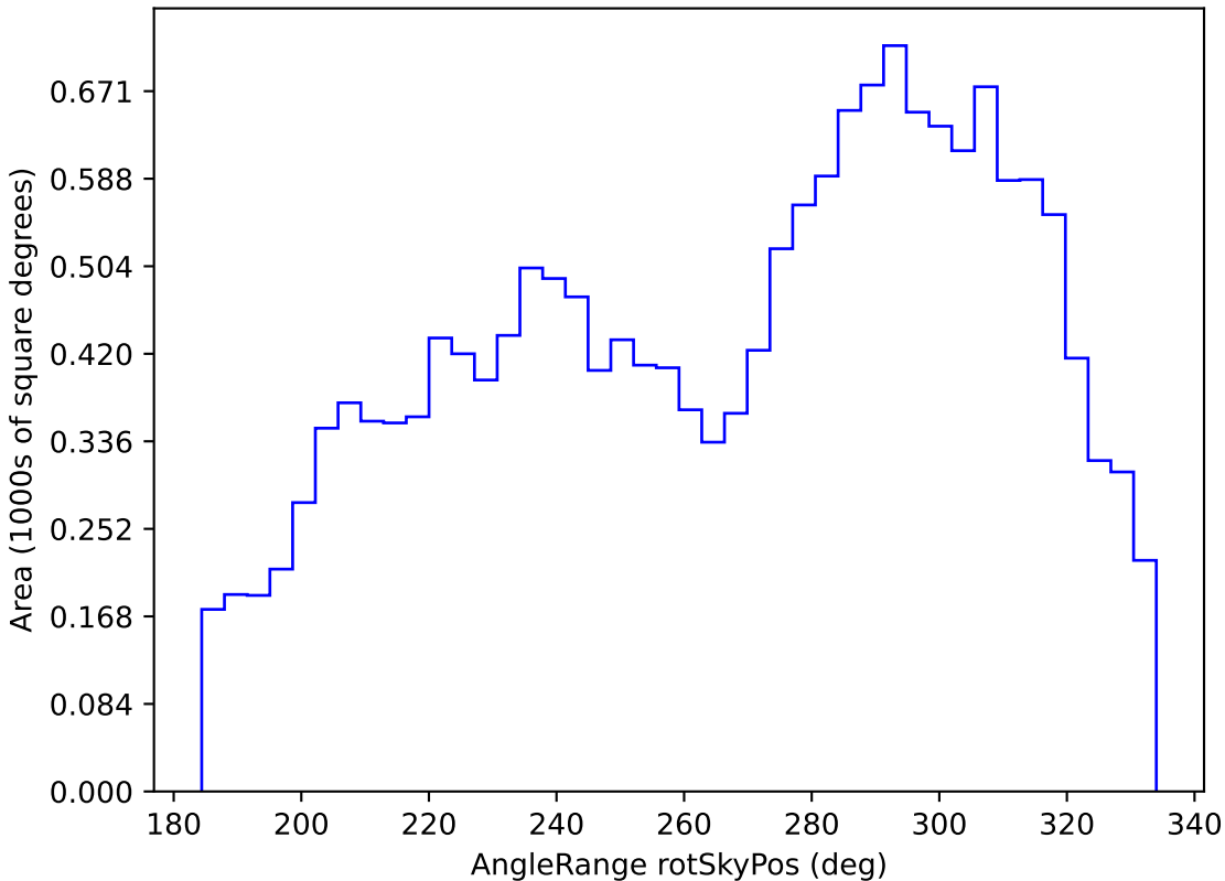
too_5_1v3.4_10yrs WFD g band: AngleRange rotSkyPos
