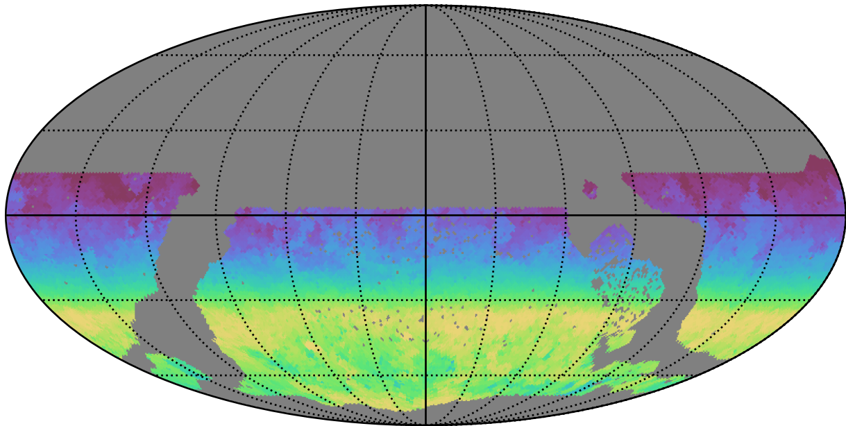
too_5_1v3.4_10yrs WFD all bands: AngleRange rotSkyPos
