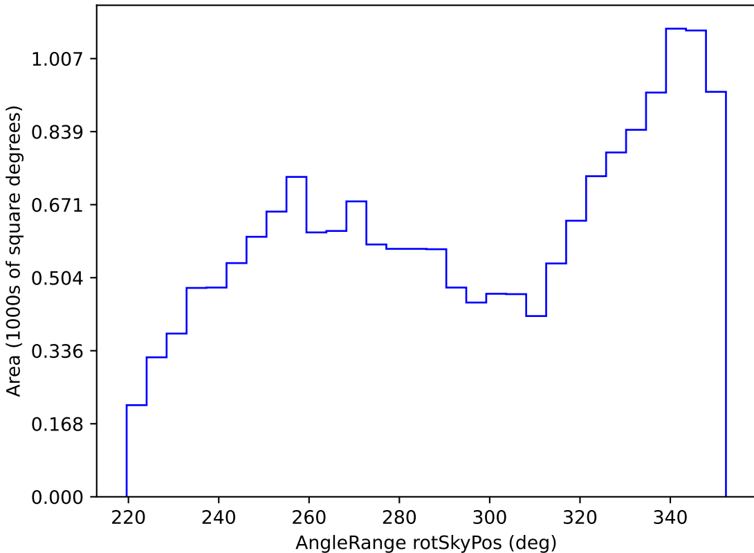
too_5_1v3.4_10yrs WFD all bands: AngleRange rotSkyPos
