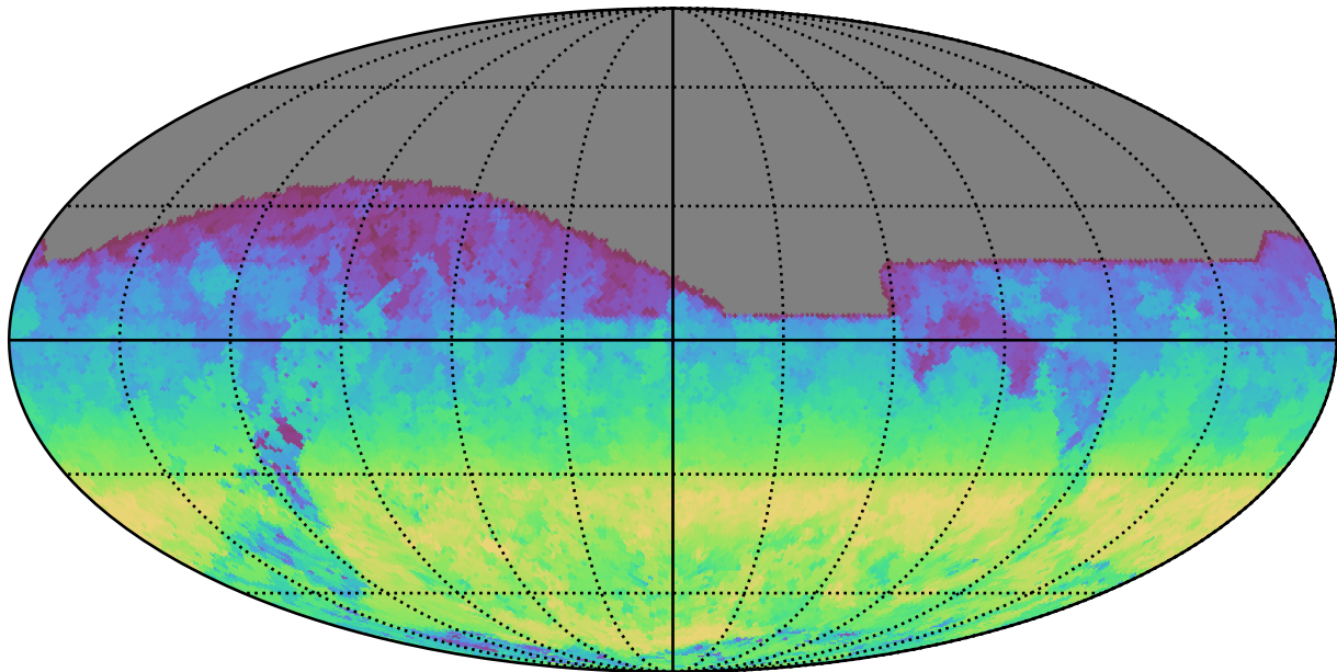
too_5_1v3.4_10yrs All sky z band: AngleRange rotSkyPos
