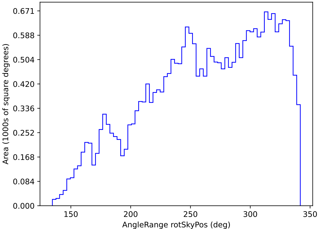
too_5_1v3.4_10yrs All sky z band: AngleRange rotSkyPos
