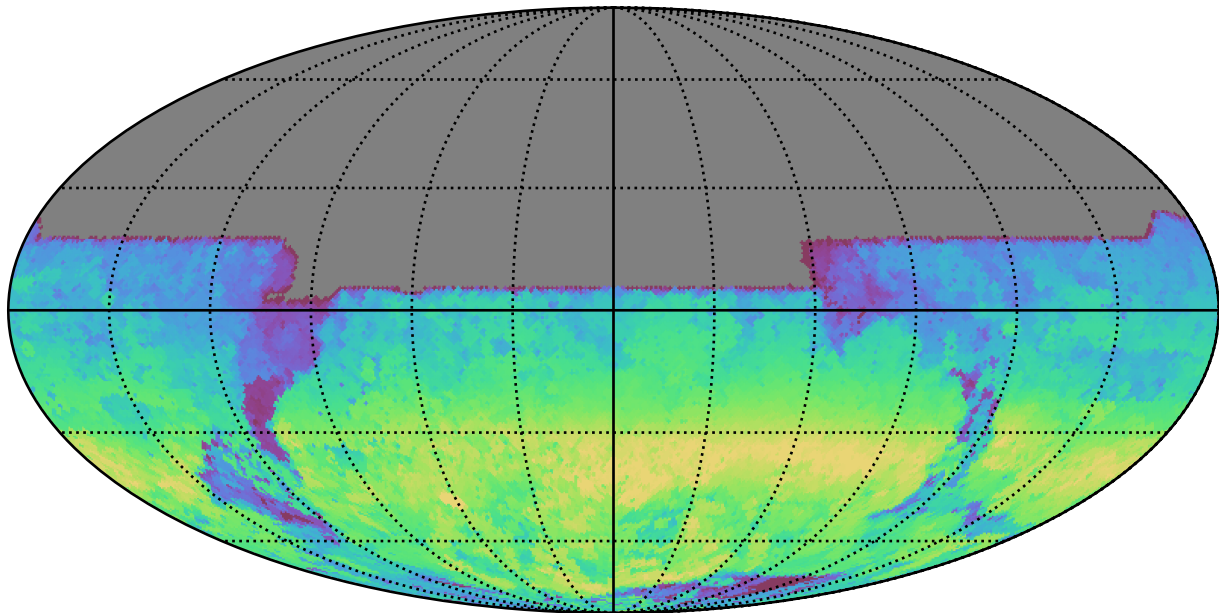
too_5_1v3.4_10yrs All sky y band: AngleRange rotSkyPos
