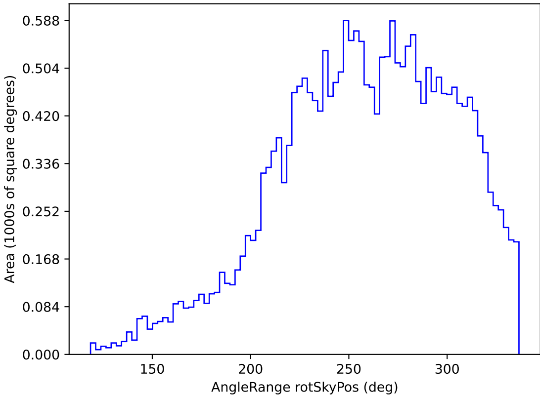
too_5_1v3.4_10yrs All sky y band: AngleRange rotSkyPos
