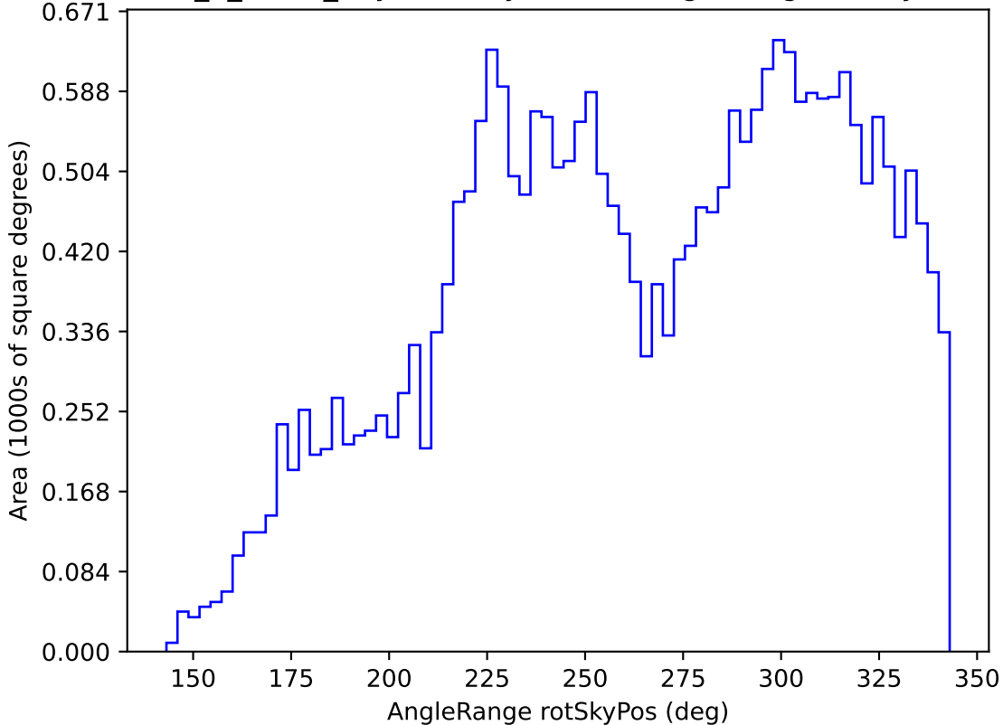
too_5_1v3.4_10yrs All sky r band: AngleRange rotSkyPos
