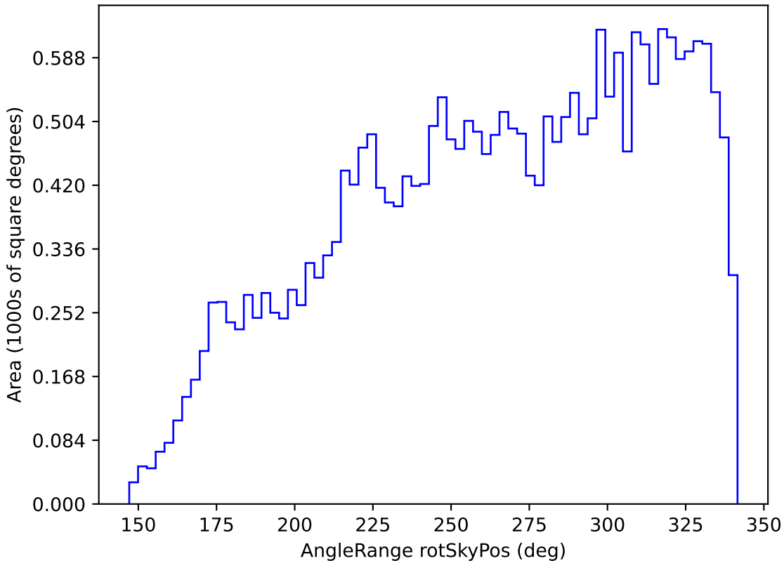
too_5_1v3.4_10yrs All sky i band: AngleRange rotSkyPos
