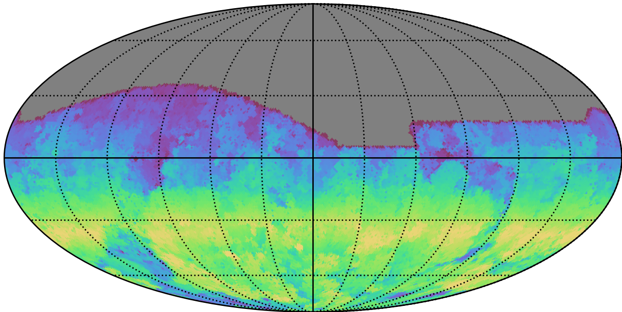
too_5_1v3.4_10yrs All sky g band: AngleRange rotSkyPos
