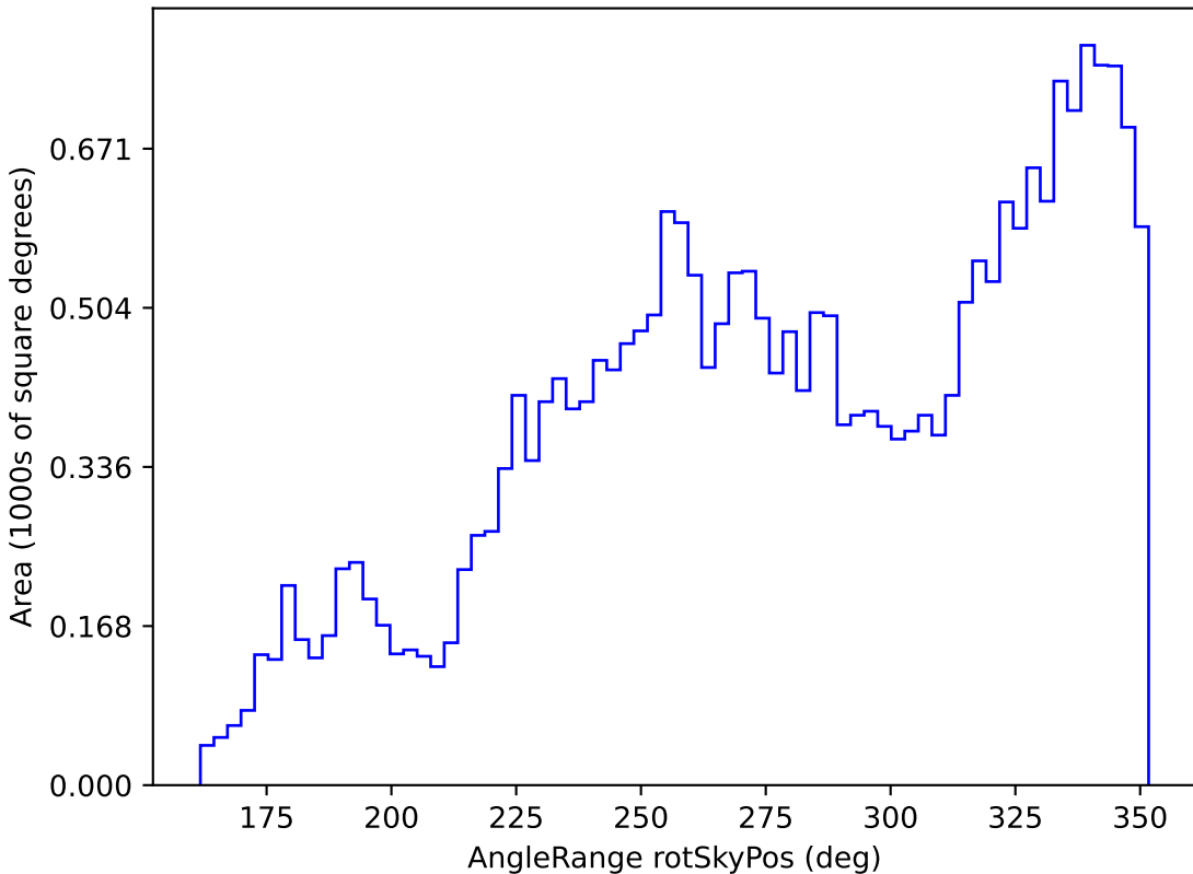
too_5_1v3.4_10yrs All sky all bands: AngleRange rotSkyPos
