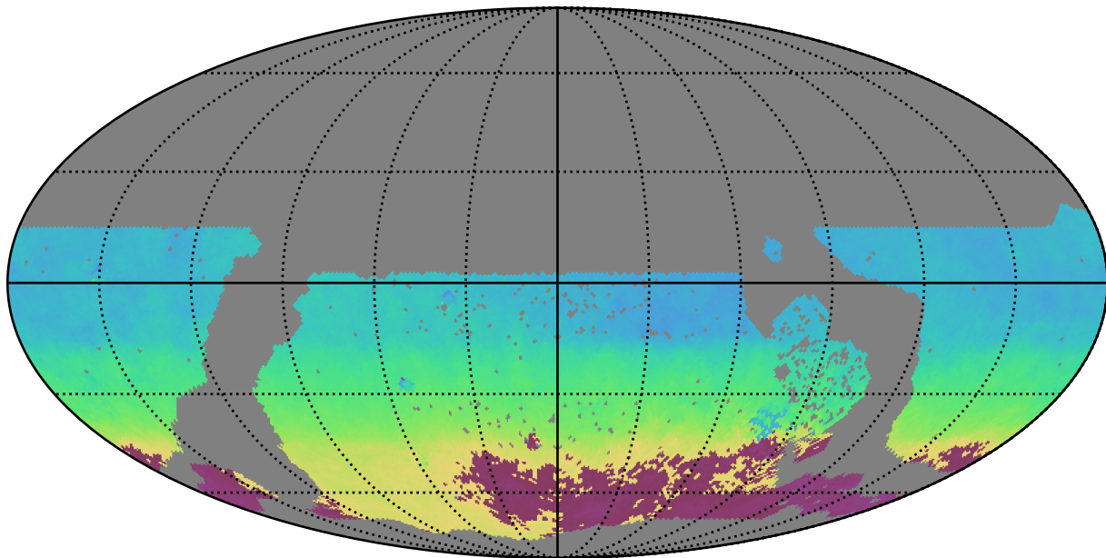
too_5_1v3.4_10yrs WFD z band: AngleMean rotSkyPos
