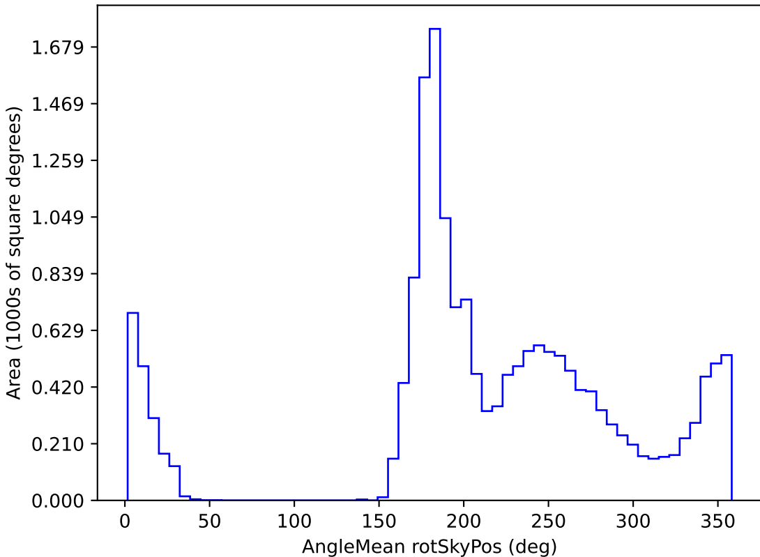
too_5_1v3.4_10yrs WFD z band: AngleMean rotSkyPos
