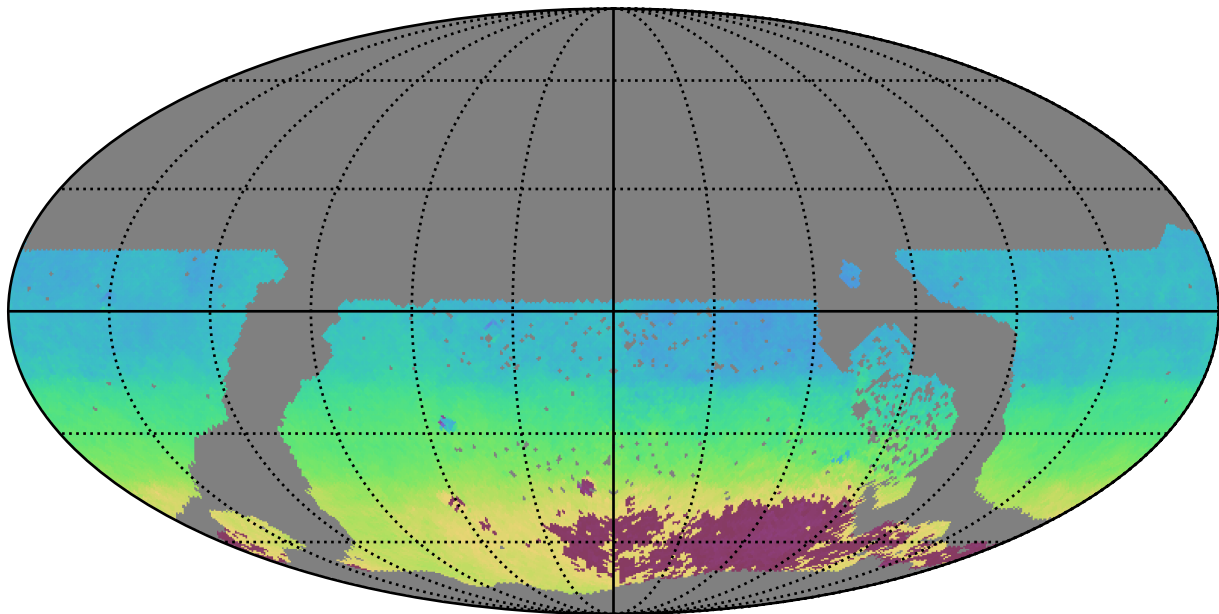
too_5_1v3.4_10yrs WFD y band: AngleMean rotSkyPos
