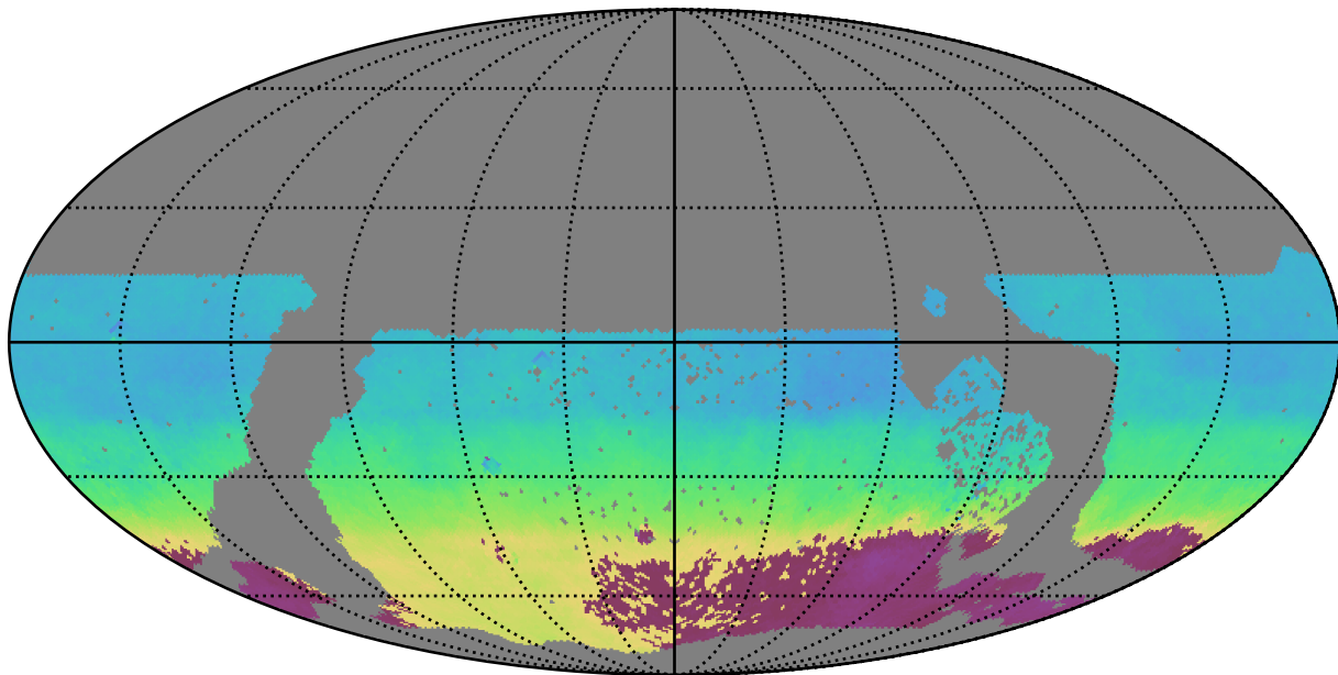
too_5_1v3.4_10yrs WFD r band: AngleMean rotSkyPos
