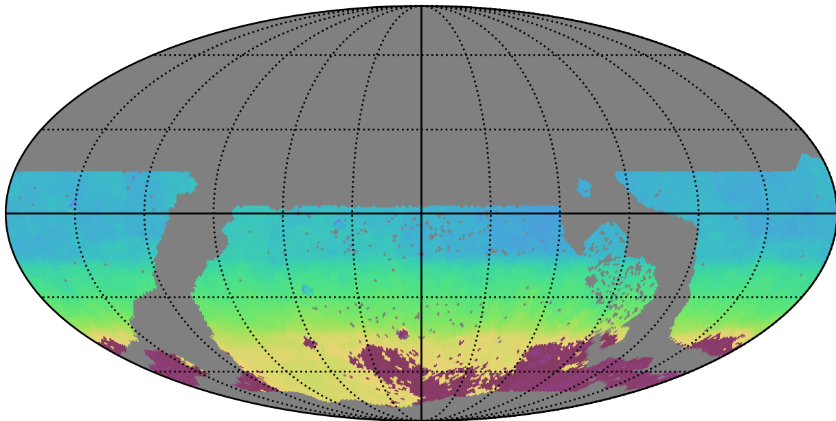
too_5_1v3.4_10yrs WFD i band: AngleMean rotSkyPos
