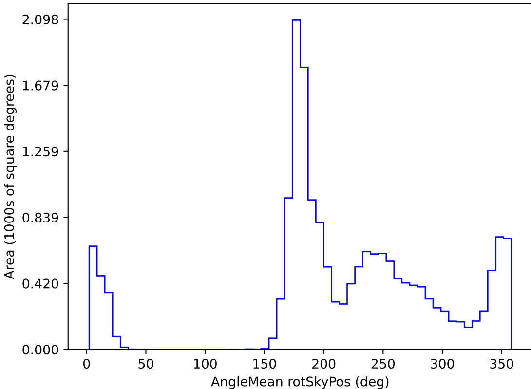
too_5_1v3.4_10yrs WFD i band: AngleMean rotSkyPos
