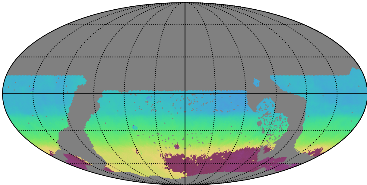
too_5_1v3.4_10yrs WFD all bands: AngleMean rotSkyPos
