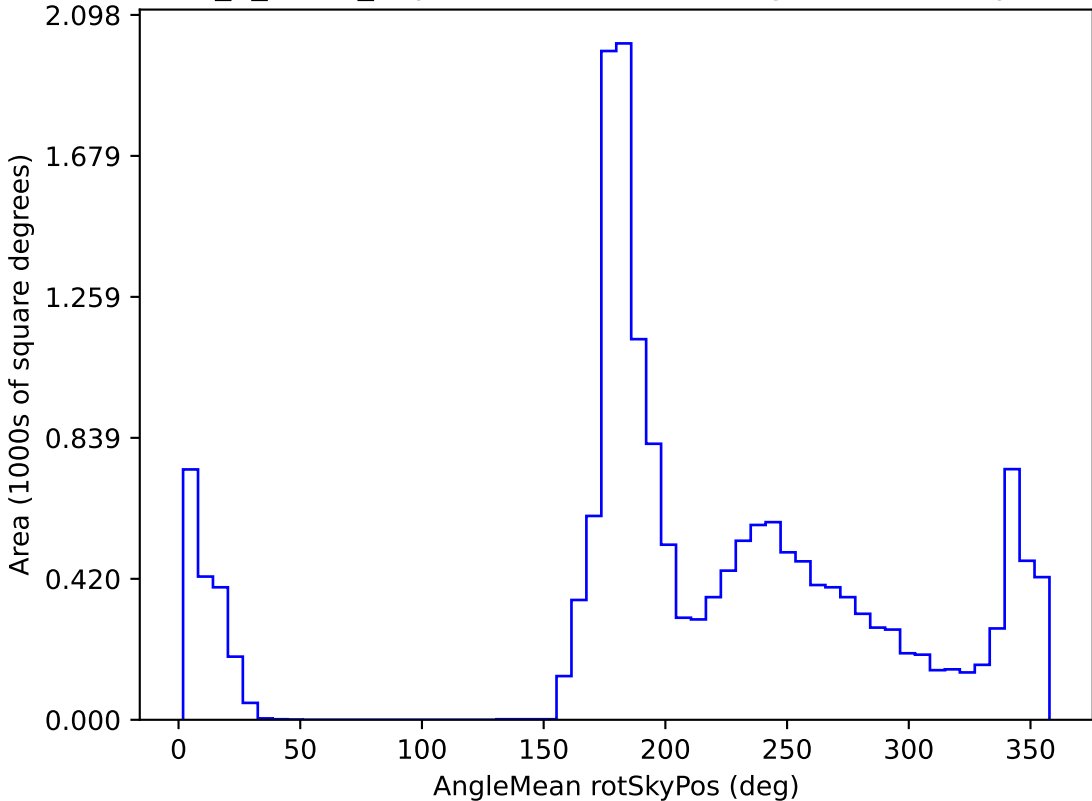
too_5_1v3.4_10yrs WFD all bands: AngleMean rotSkyPos
