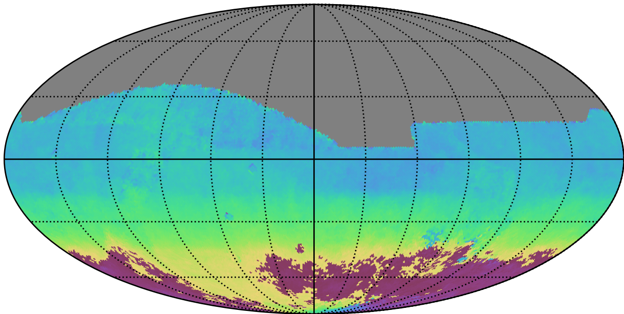
too_5_1v3.4_10yrs All sky z band: AngleMean rotSkyPos
