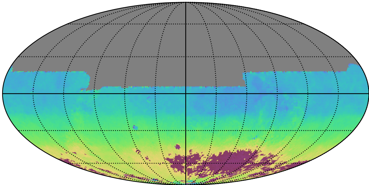
too_5_1v3.4_10yrs All sky y band: AngleMean rotSkyPos
