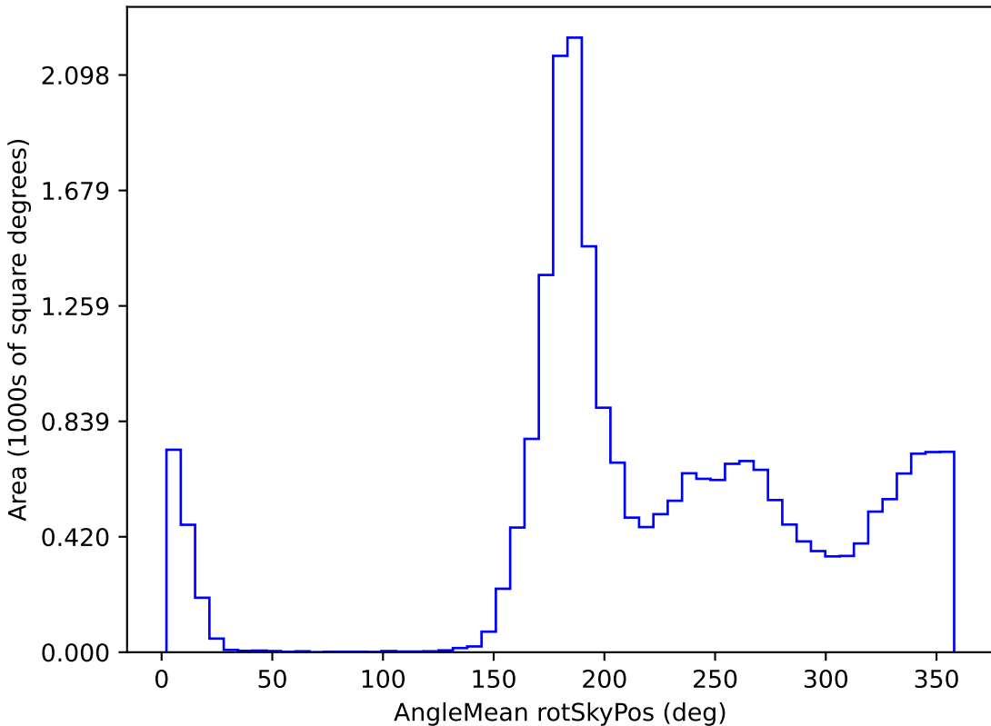
too_5_1v3.4_10yrs All sky y band: AngleMean rotSkyPos
