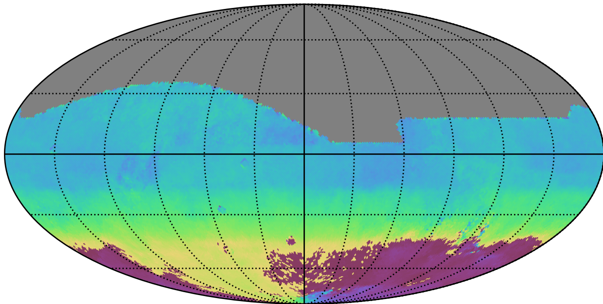
too_5_1v3.4_10yrs All sky r band: AngleMean rotSkyPos
