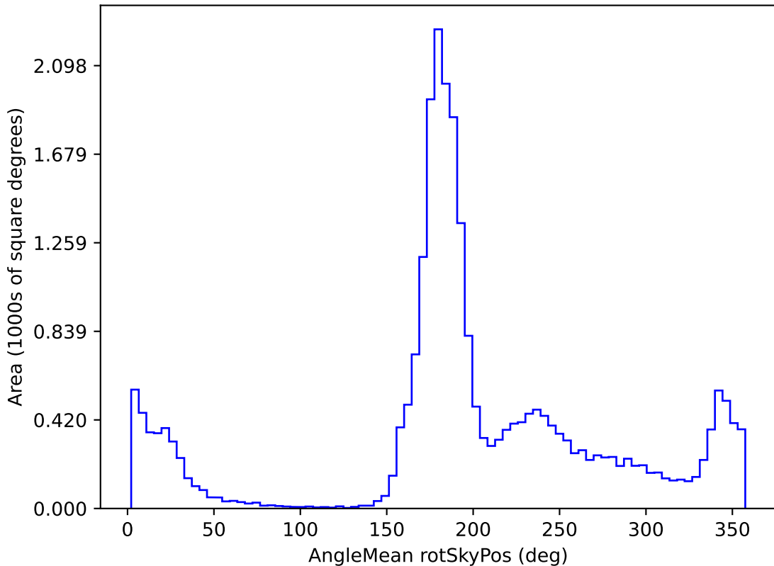
too_5_1v3.4_10yrs All sky r band: AngleMean rotSkyPos
