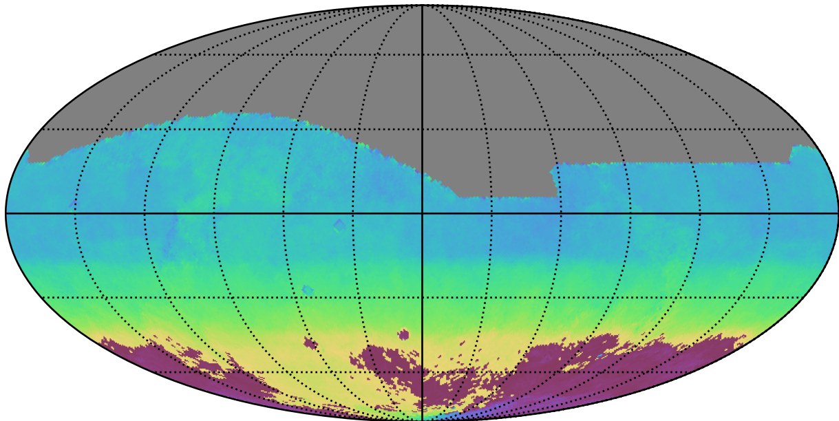
too_5_1v3.4_10yrs All sky i band: AngleMean rotSkyPos
