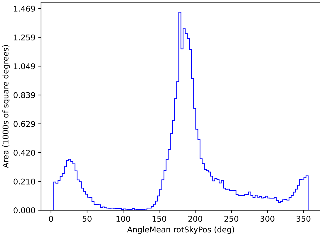
too_5_1v3.4_10yrs All sky g band: AngleMean rotSkyPos
