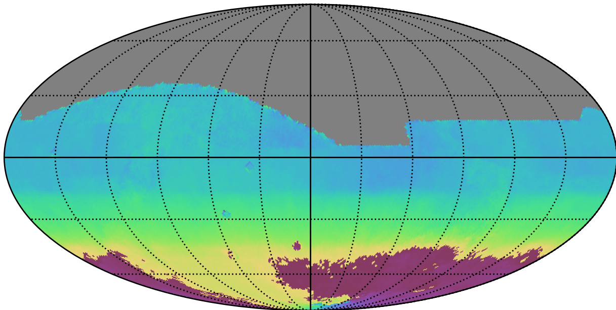
too_5_1v3.4_10yrs All sky all bands: AngleMean rotSkyPos
