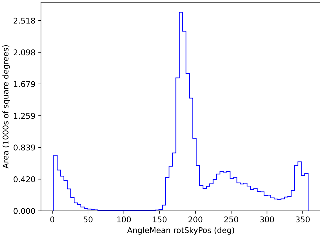
too_5_1v3.4_10yrs All sky all bands: AngleMean rotSkyPos
