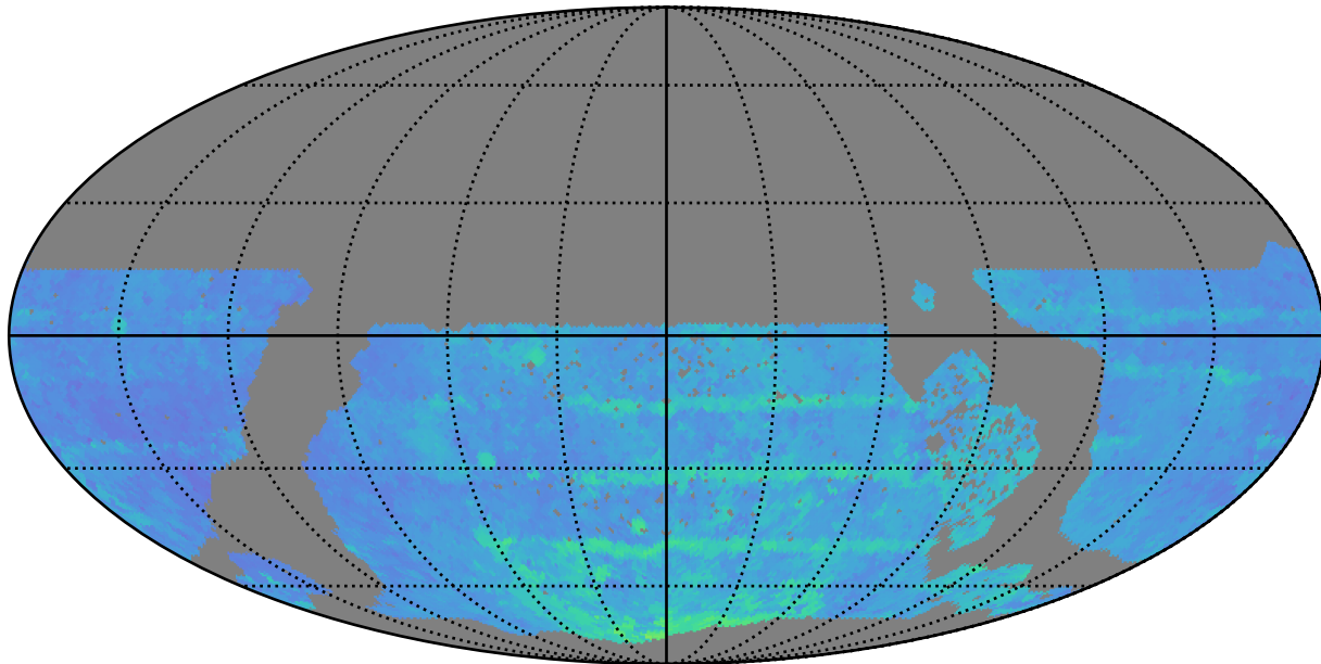
too_5_1v3.4_10yrs WFD z band: 80thPercentile Season Length
