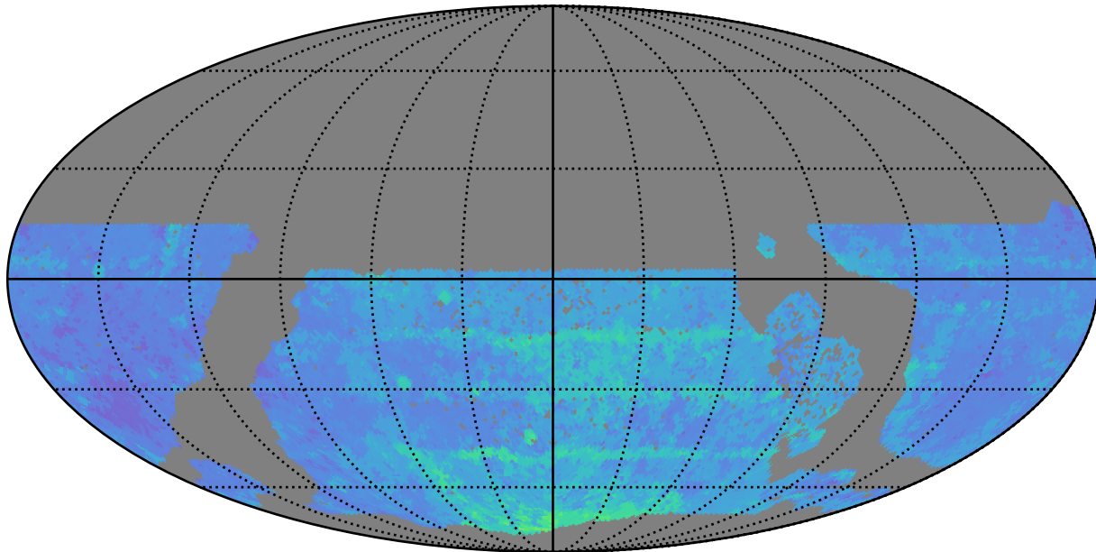
too_5_1v3.4_10yrs WFD y band: 80thPercentile Season Length
