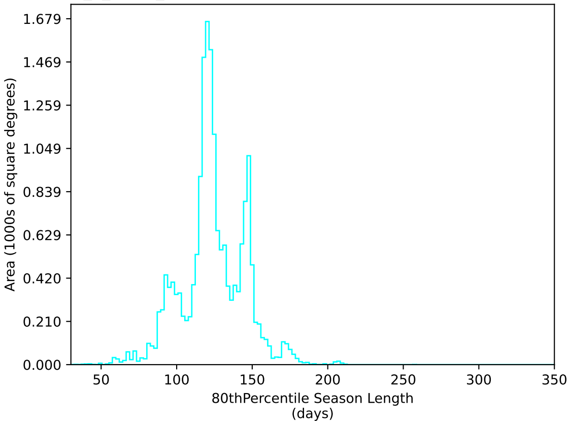
too_5_1v3.4_10yrs WFD u band: 80thPercentile Season Length
