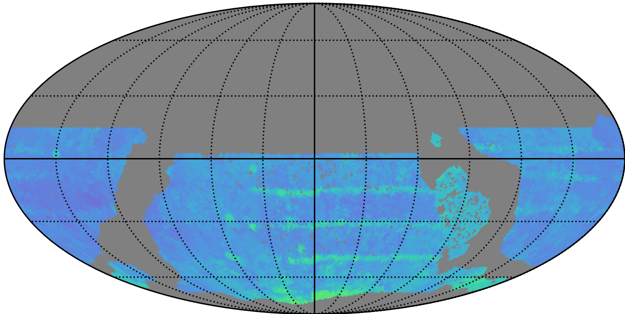
too_5_1v3.4_10yrs WFD r band: 80thPercentile Season Length
