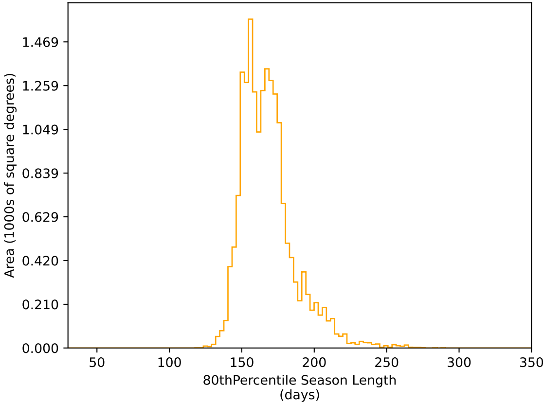
too_5_1v3.4_10yrs WFD r band: 80thPercentile Season Length
