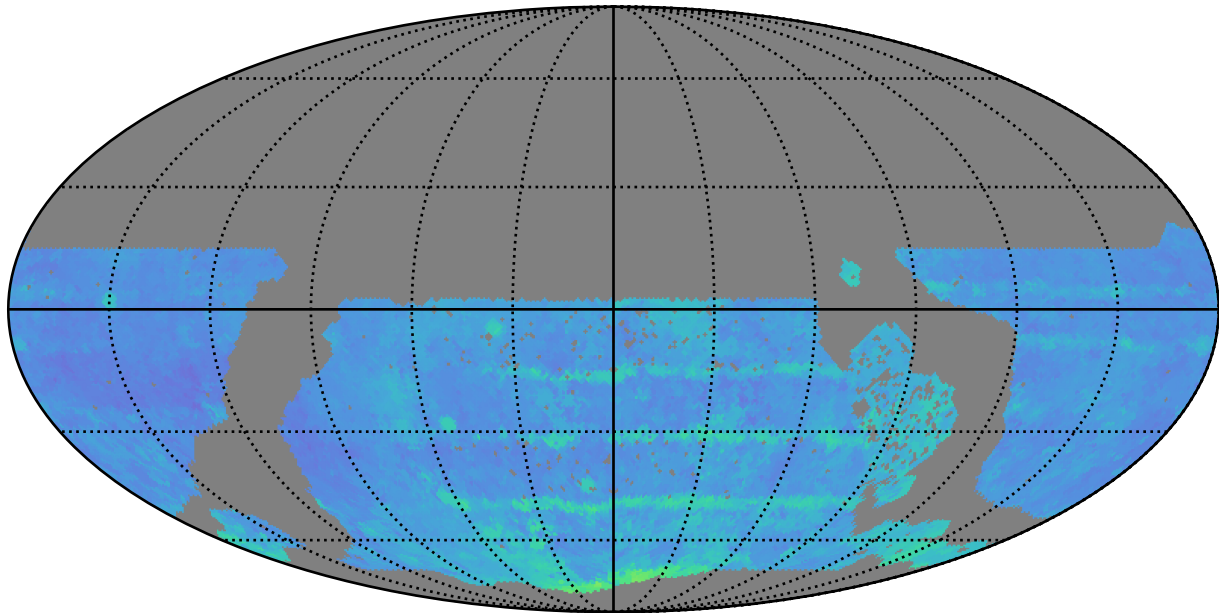
too_5_1v3.4_10yrs WFD i band: 80thPercentile Season Length
