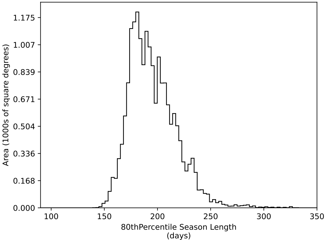
too_5_1v3.4_10yrs WFD all bands: 80thPercentile Season Length
