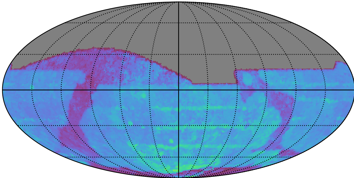
too_5_1v3.4_10yrs All sky z band: 80thPercentile Season Length
