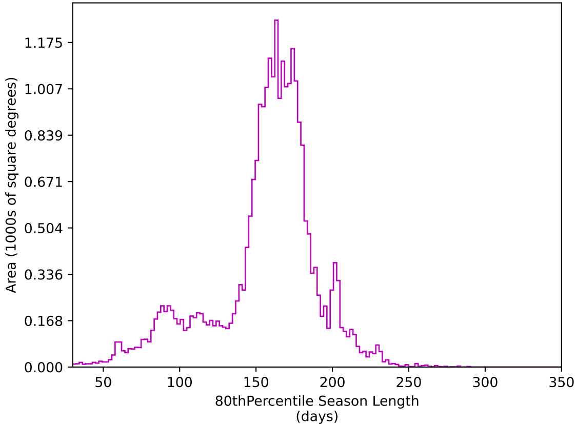
too_5_1v3.4_10yrs All sky z band: 80thPercentile Season Length
