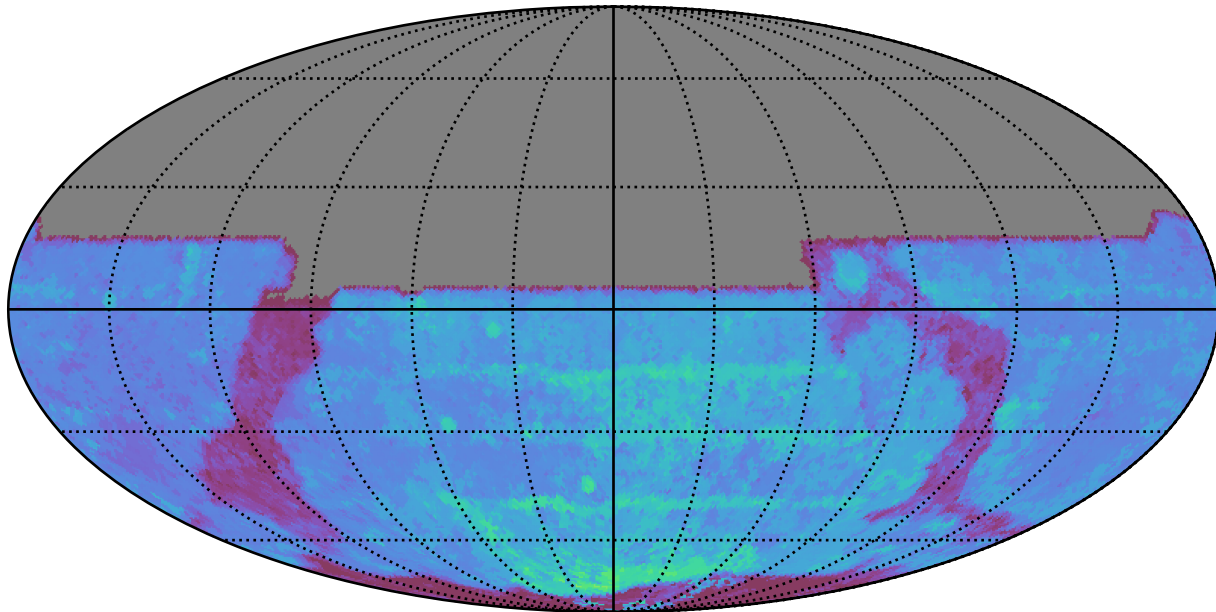
too_5_1v3.4_10yrs All sky y band: 80thPercentile Season Length
