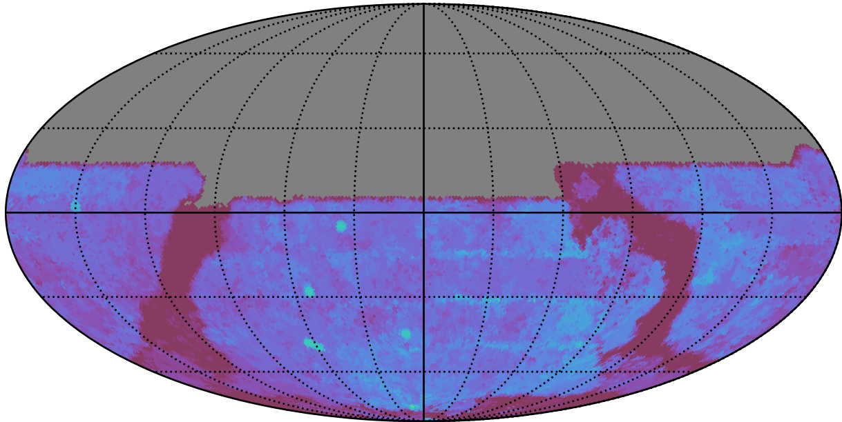
too_5_1v3.4_10yrs All sky u band: 80thPercentile Season Length
