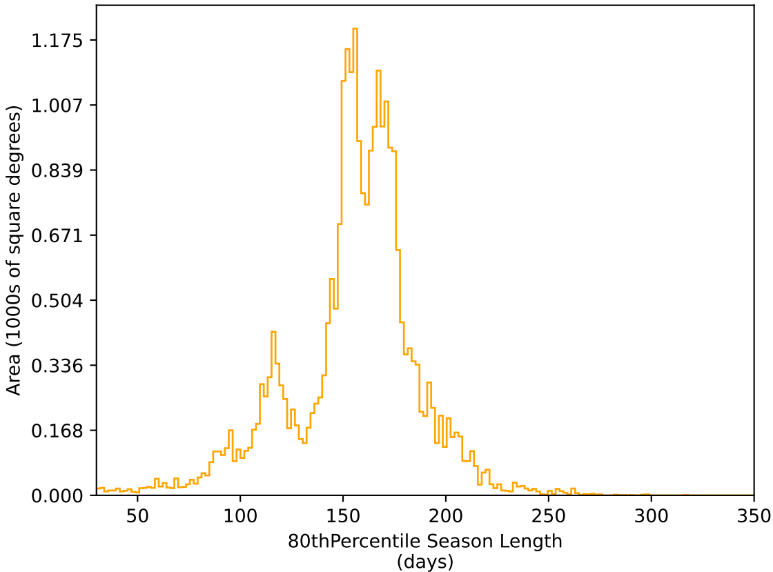
too_5_1v3.4_10yrs All sky r band: 80thPercentile Season Length
