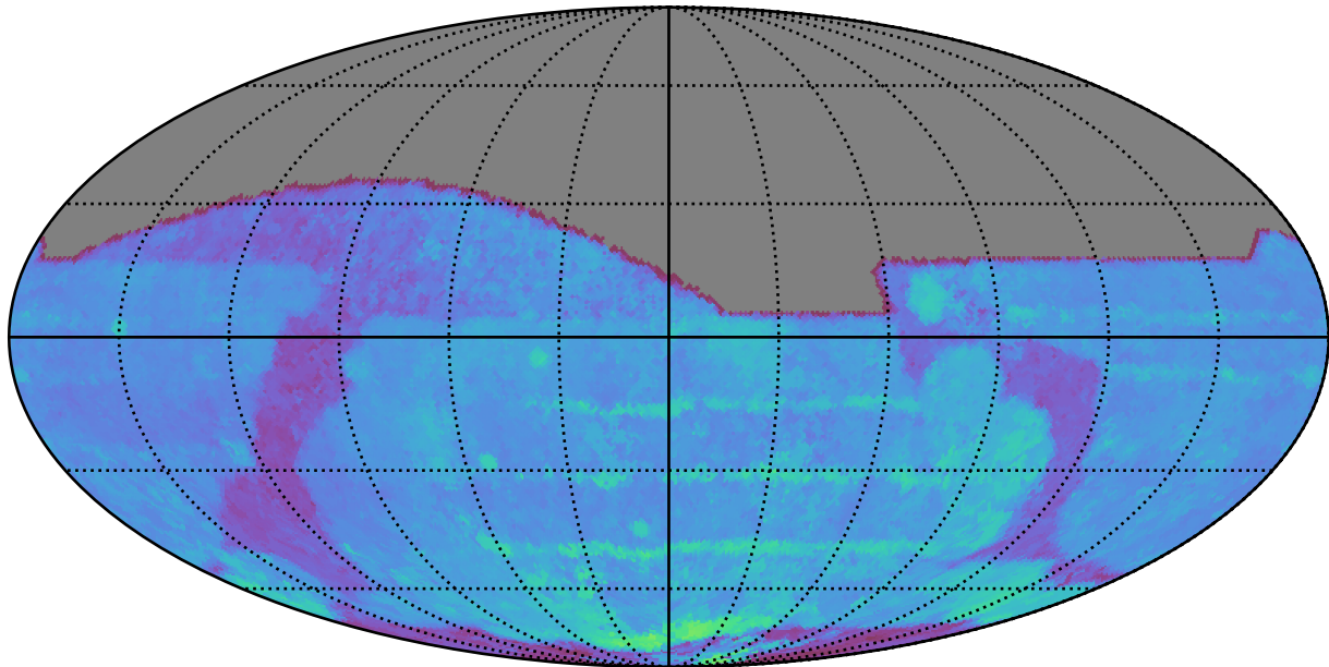
too_5_1v3.4_10yrs All sky i band: 80thPercentile Season Length
