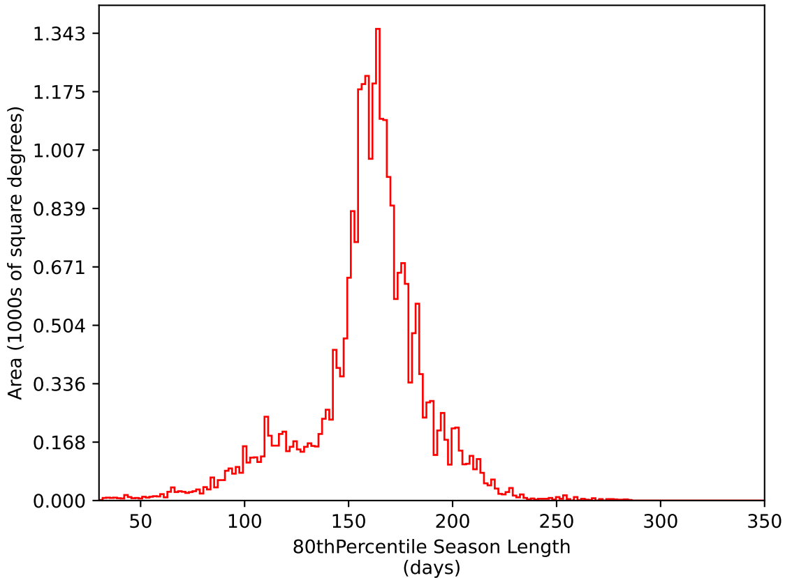
too_5_1v3.4_10yrs All sky i band: 80thPercentile Season Length
