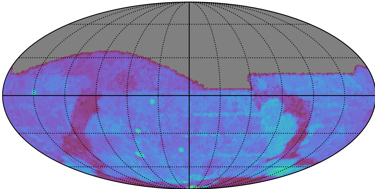
too_5_1v3.4_10yrs All sky g band: 80thPercentile Season Length
