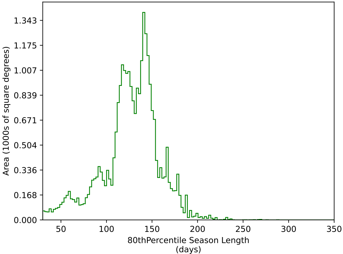
too_5_1v3.4_10yrs All sky g band: 80thPercentile Season Length
