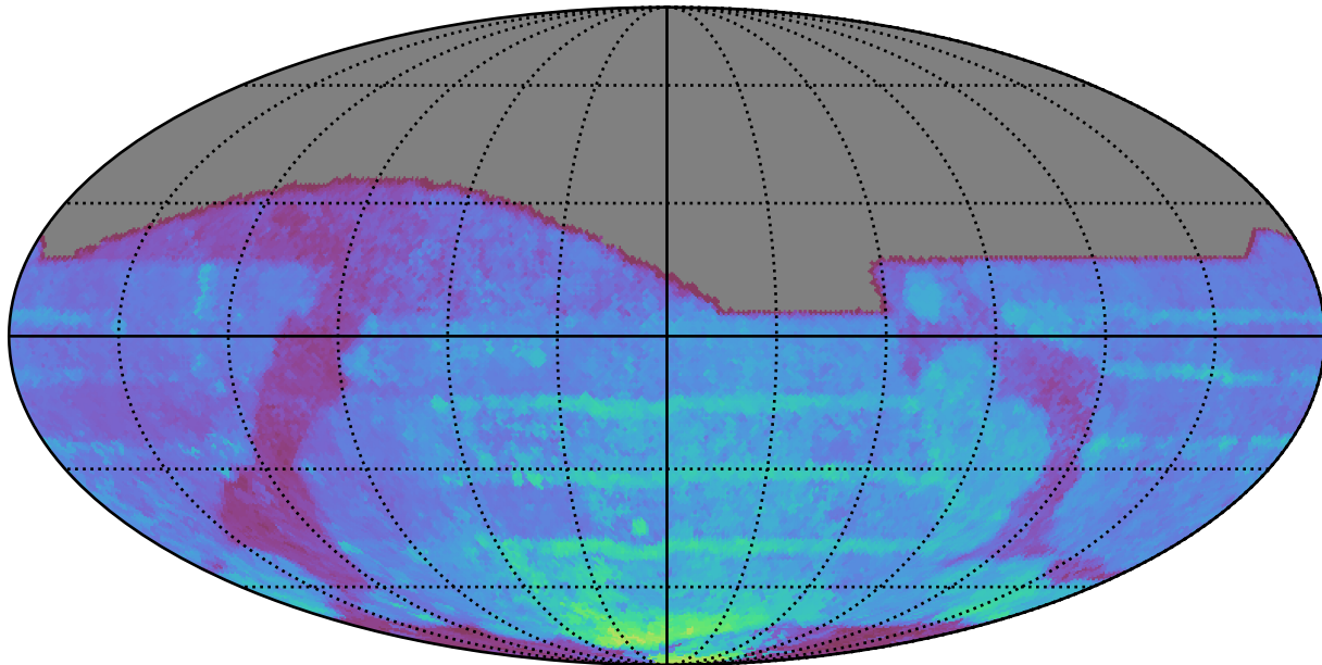
too_5_1v3.4_10yrs All sky all bands: 80thPercentile Season Length
